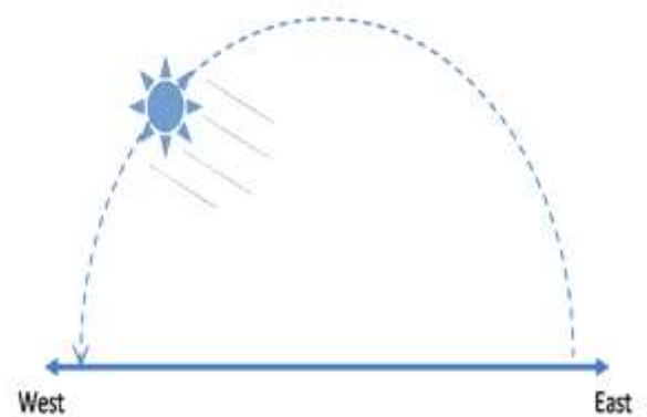
Fig.1. The Sun's Track
