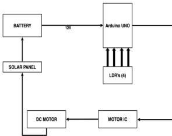
Fig.3. Block Diagram for Dual-Axis Tracker.
