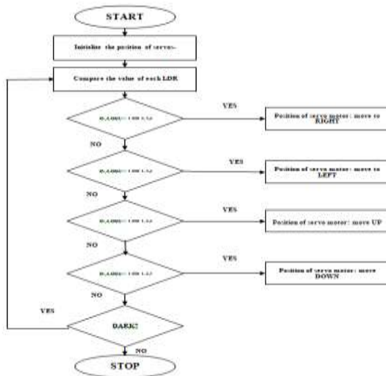
Fig.4.Flowchart of the software program
