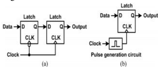
Fig.1. (a) Master-slave flip-flop (b) Pulsed latch
