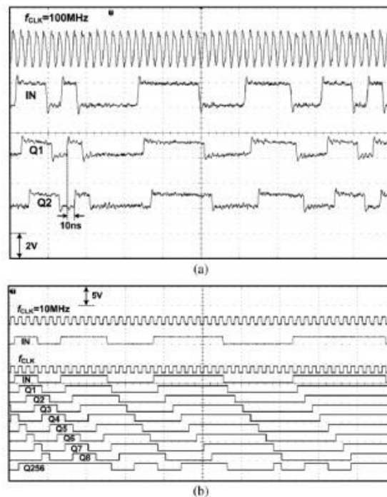
Fig.5. Measured waveforms of the proposed shift-register at (a) f_{CLK}=100\text{MHz} ; (b) f_{CLK}=10\text{MHz} .
