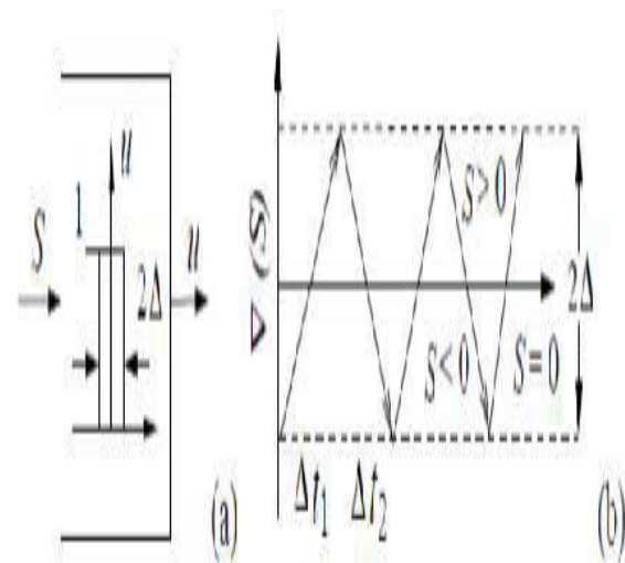
Fig. 9 Schematic diagram showing the: (a) hysteresis function; and (b) the state trajectory in the vicinity of sliding surface S = 0 .
