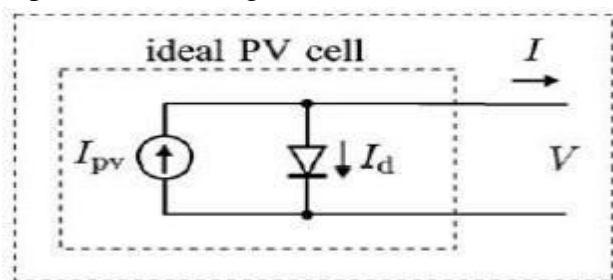
Fig. 4 Equivalent circuit of ideal PV cell with R_p and R_s
