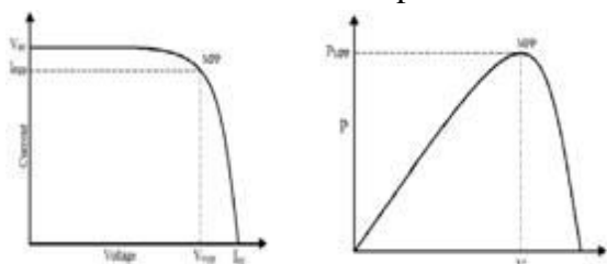
Fig. 5 I-V and P-V characteristics of PV cell
