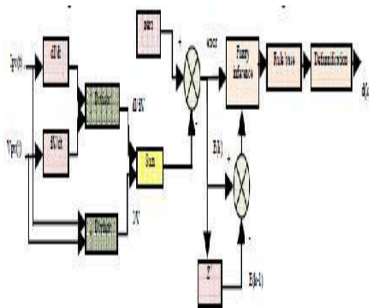
Fig. 8 Fuzzy logic based scheme for MPP tracking
