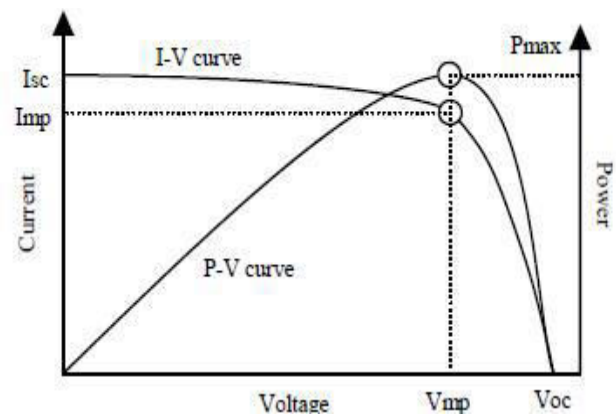
Fig. 2 Current-voltage and power-voltage characteristics of a solar cell
