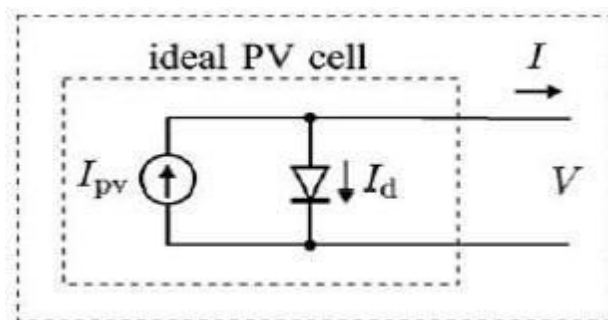
Fig. 3 Equivalent circuit of ideal PV cell
