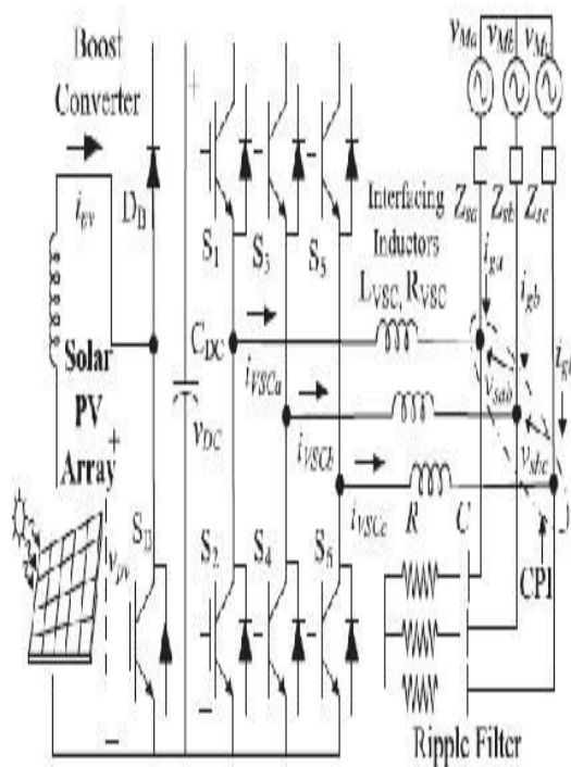
Fig. 1 System Configuration
