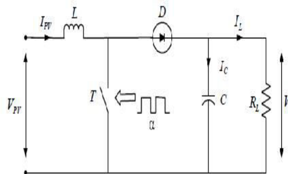
Fig. 6 Equivalent circuit of a boost converter
