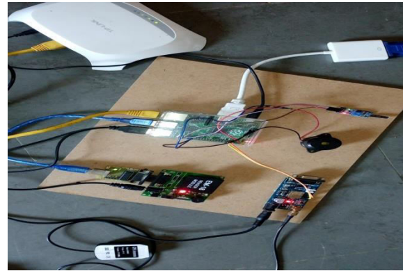
Fig 7. Hardware setup in the vehicle
