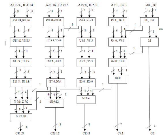
Fig.4: 32-bit Efficient Ladner-Fischer Adder
