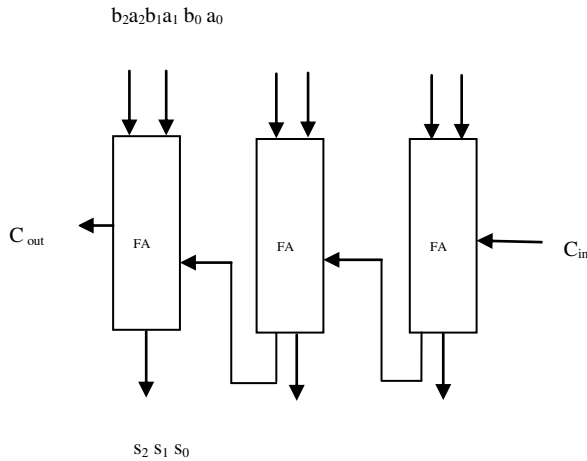
Fig.1: Three Bit Ripple Carry Adder
