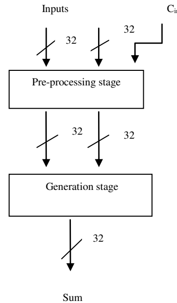
Fig.2: Block Diagram
