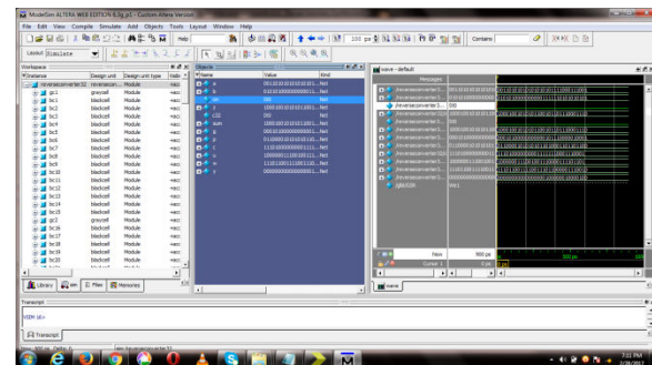
Fig.5: 32-Bit Efficient Ladner-Fischer Adder Simulation Waveform
