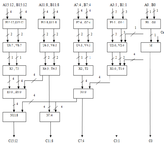
Fig.3: 16-Bit Efficient Ladner-Fischer Adder
