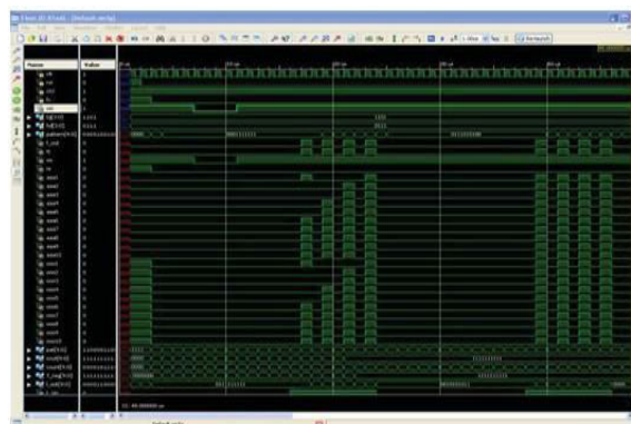
Fig 10:Simulation result of LP decompressor
