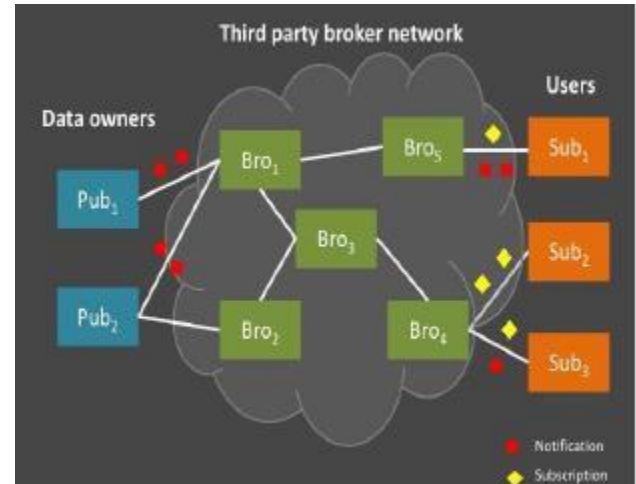
Fig 1. Subscriber/Publisher System
