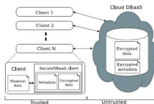
Fig. 1. SecureDBaaS architecture.
