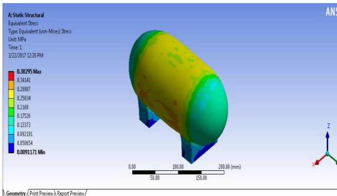
Figure 5.2 shows the equivalent stress analysis on pressure vessel of stainless steel material
