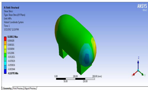
Figure 5.3 shows the shear stress of pressure vessel of stainless steel material
