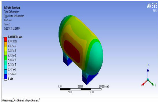
Figure 5.1 shows the Total deformation of the pressure vessel formed with stainless steel material
