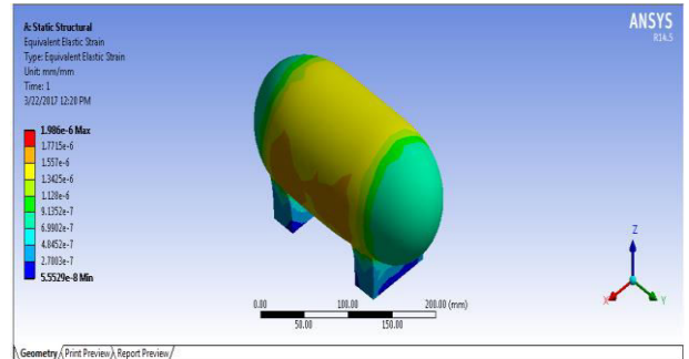
Figure 5.4 shows the Equivalent Elastic strain of pressure vessel of stainless steel material
