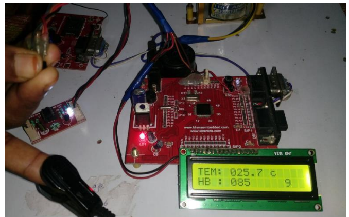
Figure 9. Implemented circuit (Showing output)
