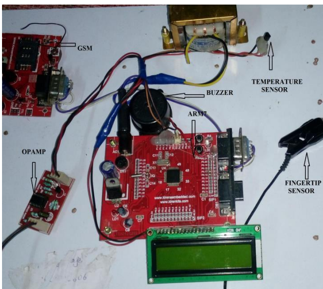
Figure 7. Implemented system for Heart rate and temperature measurement
