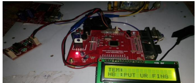
Figure 8. Implemented circuit (Ready to measure)
