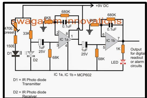
Figure 4. Schematic of heart rate conditioning circuit
