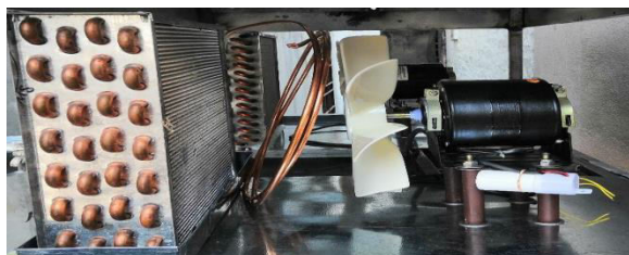
Figure: Evaporator and fan fitting.
