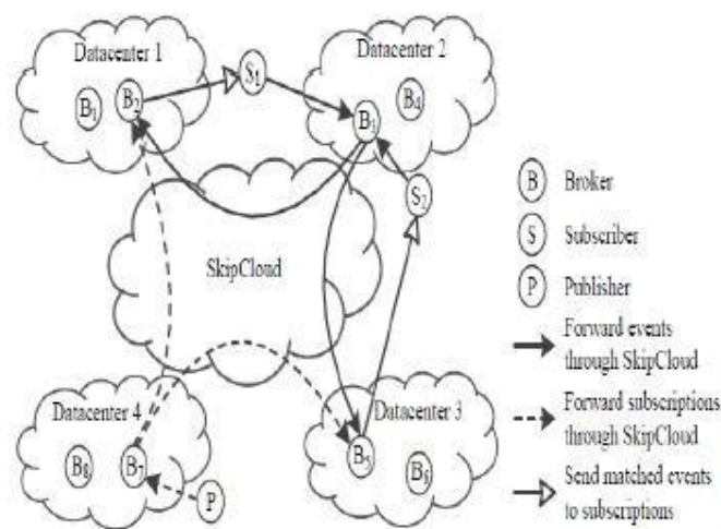
Fig. 2. System Architecture.
