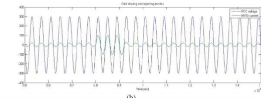
Fig.6 Grid sharing and grid injecting modes of operation (b) PCC voltage and MVSI current
