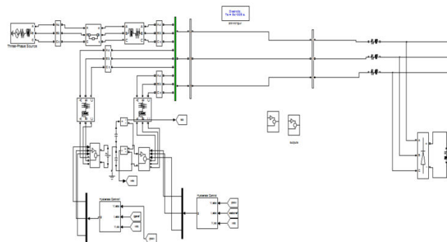
Fig.2 Simulation model of the DVSI scheme.
