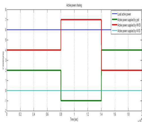
Fig.3 Active power sharing
