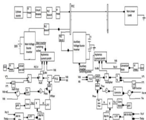
Fig.1 Control strategy of DVSI scheme
