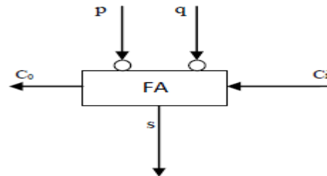
Fig. 2 Boolean equation and schematics for half adder even bit
